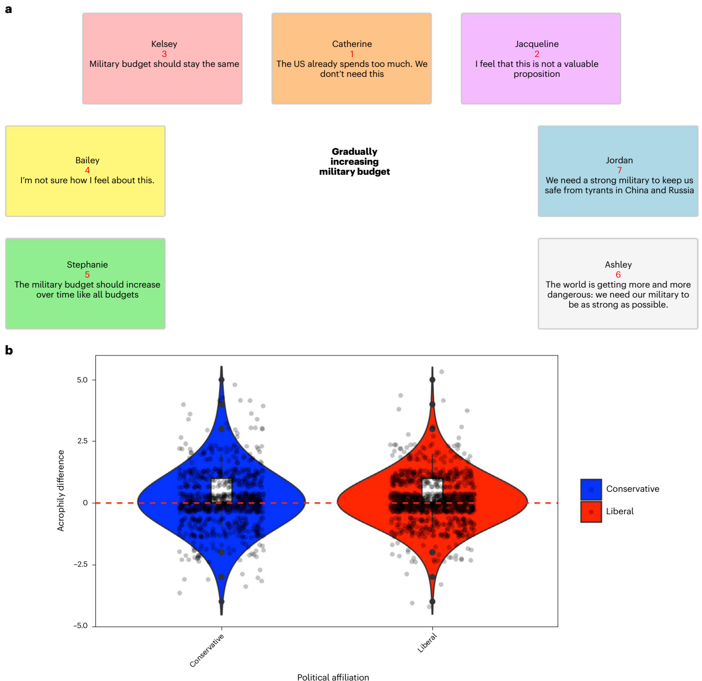
Fig. 5 | Task and results of study 4. a. Representative peer rating window from which participants were asked to choose one peer they would like to keep. b. Acrophily difference between participants and the peer they chose to keep in response to each concept ( N = 386 ). Positive values represent acrophily, and
